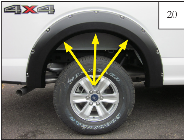
Press flares firmly onto the vehicle and install and fully tighten three screws (SW1-0050) into the clips installed in step 18.
