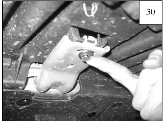
Start a factory bolt through inner structure and into brackets as shown. Note: It's easier to start bolts with your hands.
