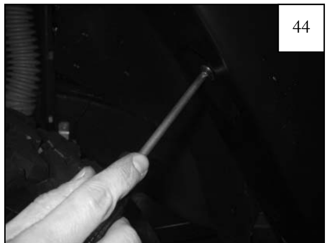
Install supplied Truss Head Screws through holes in wheel well and into #14 U-Clips installed in Step 25 (6 places). Ensure proper alignment of outer flare, inner flare and splash shield. Do not tighten at this time.
