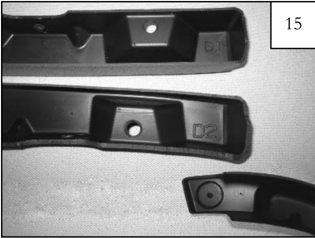
Locate the flat flare front inner pieces. The driver side front inner pieces are marked D1, D2, & D7. The passenger side front inner pieces are marked P1, P2, & P7.
