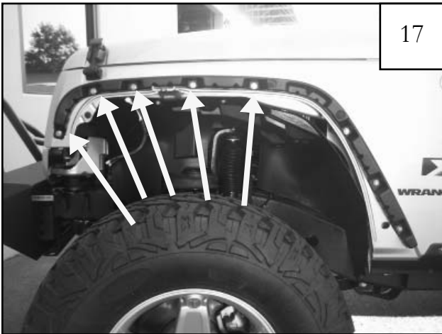
Secure inner piece D1 (and P1 for passenger side installation) to the sheet metal using the following 4 Steps: Step 1 Position inner piece on fender, aligning with existing factory holes in sheet metal.
