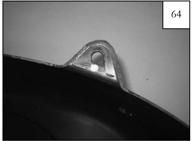
Place a grease pencil mark 1/8" below the hole on the rear mounting tab.
