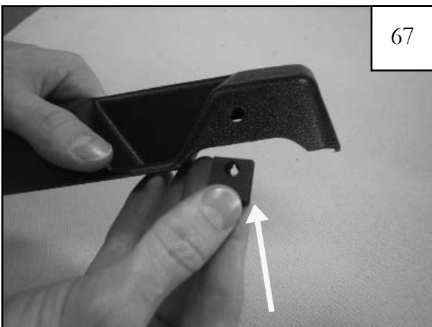
Install a speed clip at each clip location on the inner pieces, centering them on the clip location with threaded portion on inside. (6 locations) NOTE: Clips may slide out of place. Try pinching the metal tightly onto the inner piece with pliers.
