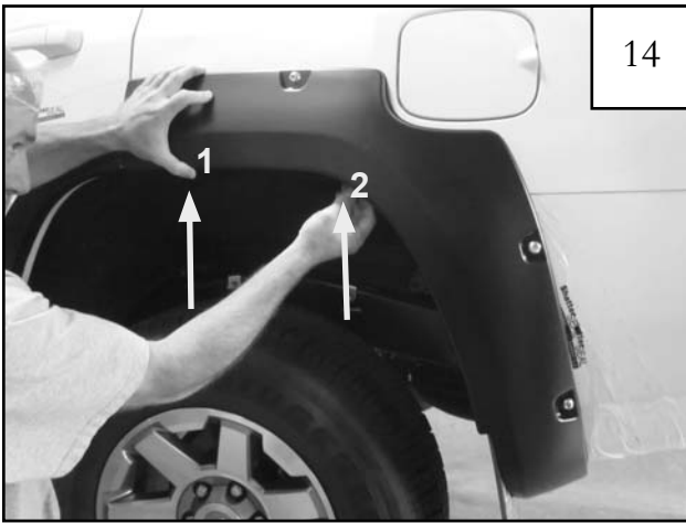
Position Flare and hand start two factory screws in to the top two holes in flare. Ensure flare is positioned properly, then apply inward pressure on the flare at each hole location while tightening each screw. NOTE: Tighten screw at the front of the flare first.
