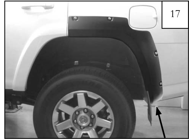
Install supplied push retainer (RV1-P009) into the lower rear hole.
