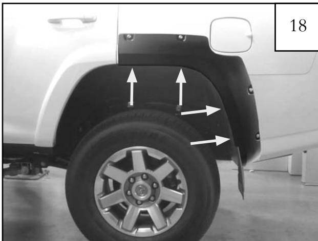
Ensure flare is positioned properly, then apply inward pressure on the flare at each hole location while tightening each screw.
