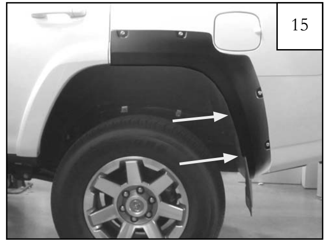
Install supplied push retainers (RV1-P009) in the two lower holes in the flare.
