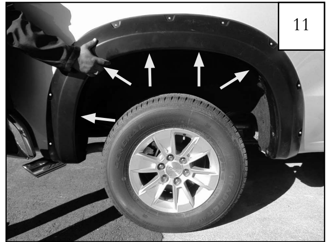
Hold flare to vehicle and install (5) supplied phillips head screws (SW1-0058) at each Clip location. Do not tighten. (If needed use an awl to align flare mounting holes.)
