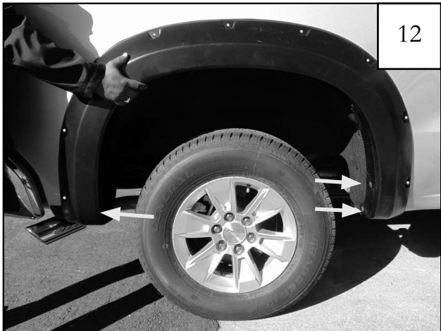
Re-install (3) factory T15 screws as indicated above. Do not tighten.
